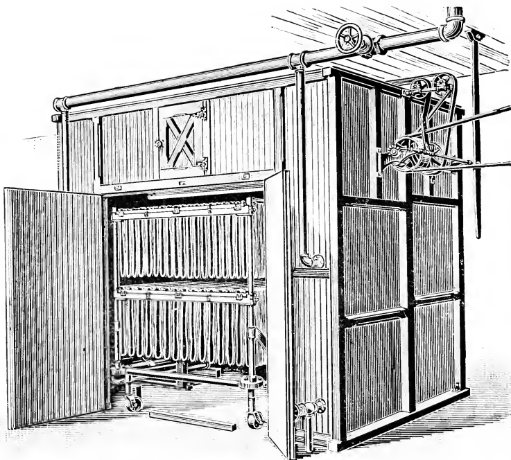
FIG. 42.—Truck Yarn-dryer.
